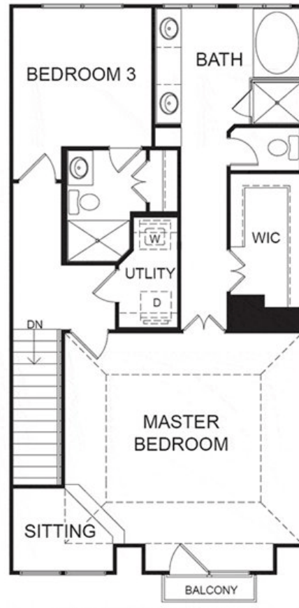
THIRD FLOOR OPT. 2
