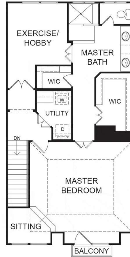
THIRD FLOOR
